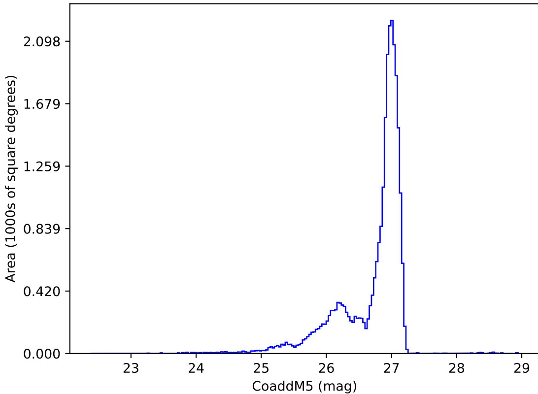
too_elab_r128_d2_griz_v3.4_10yrs r: CoaddM5
