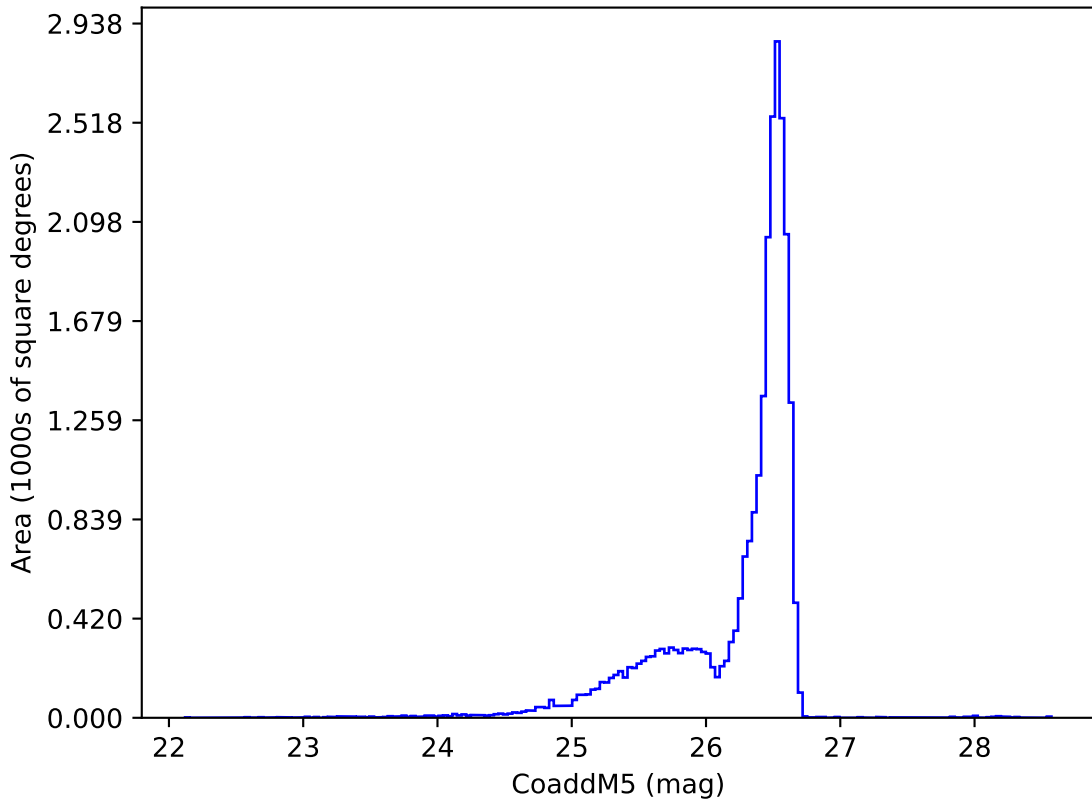
too_elab_r128_d2_griz_v3.4_10yrs i: CoaddM5
