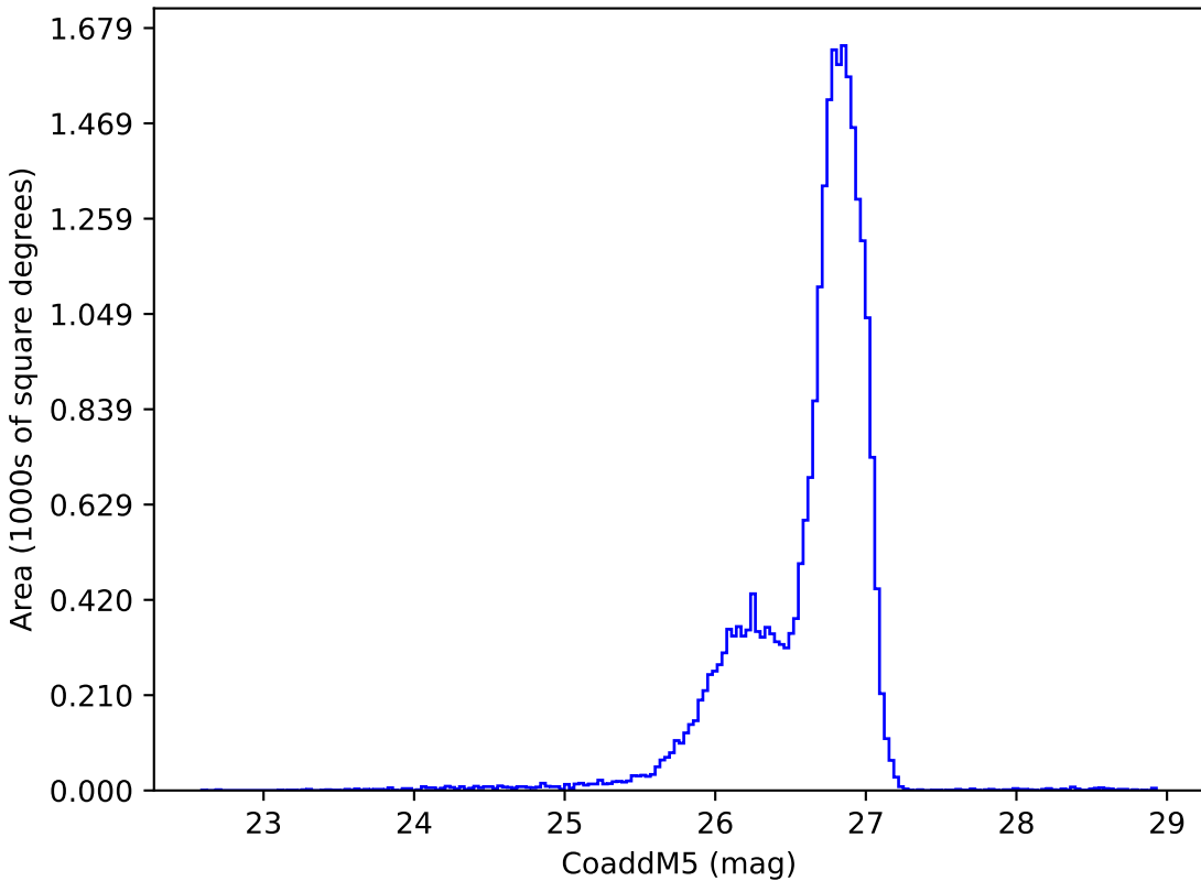
too_elab_r128_d2_griz_v3.4_10yrs g: CoaddM5
