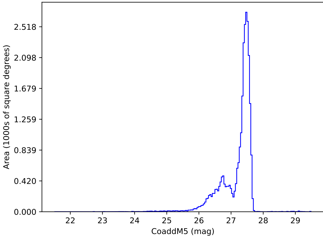
too_elab_r128_d2_griz_v3.4_10yrs : CoaddM5
