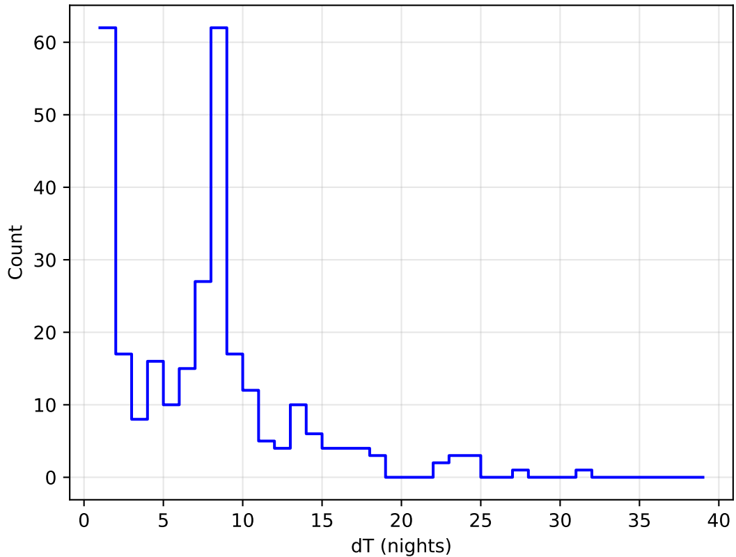
too_elab_r128_d2_griz_v3.4_10yrs all bands: DD:XMM_LSS Delta Nights Histogram
