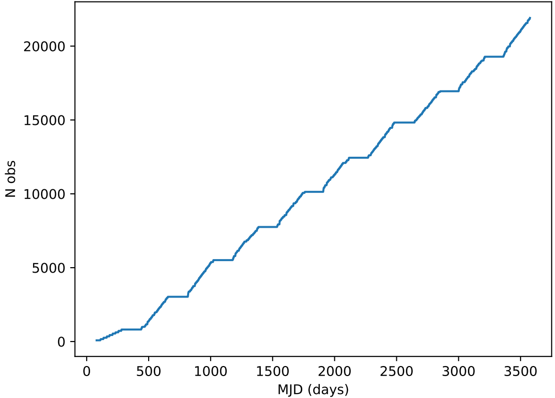
too_elab_r128_d2_griz_v3.4_10yrs all bands: DD:XMM_LSS Cumulative NVisits
