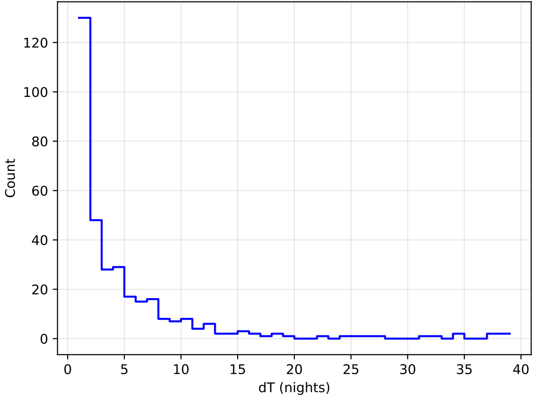
too_elab_r128_d2_griz_v3.4_10yrs all bands: DD:WFD Delta Nights Histogram
