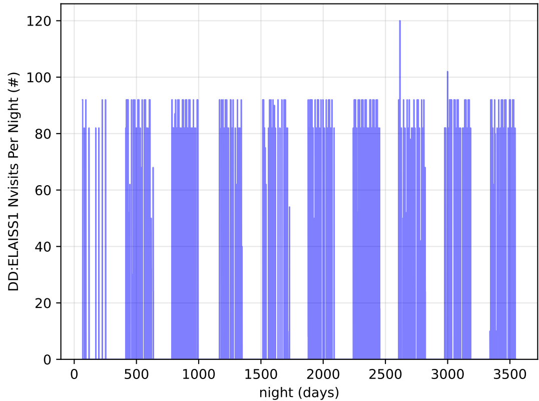
too_elab_r128_d2_griz_v3.4_10yrs all bands: DD:ELAISS1 Nvisits Per Night
