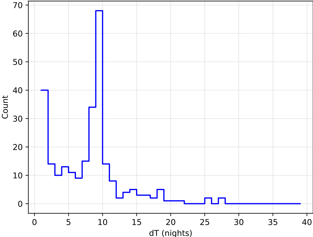
too_elab_r128_d2_griz_v3.4_10yrs all bands: DD:ELAISS1 Delta Nights Histogram
