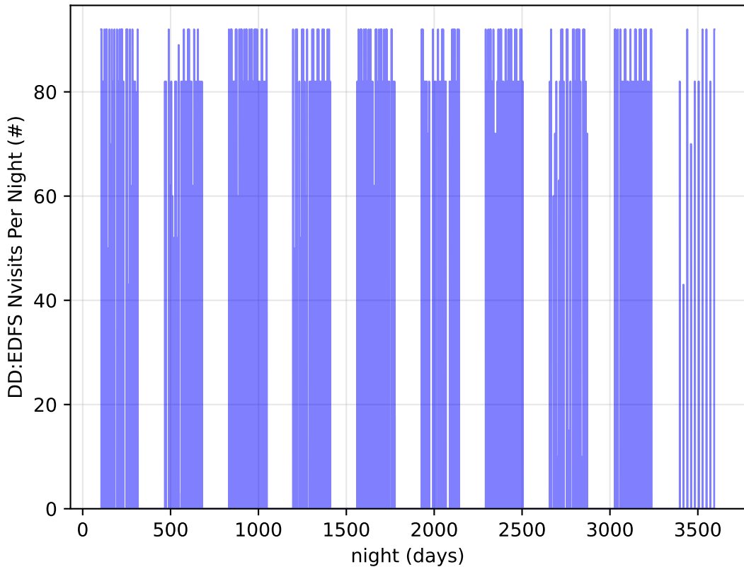
too_elab_r128_d2_griz_v3.4_10yrs all bands: DD:EDFS Nvisits Per Night
