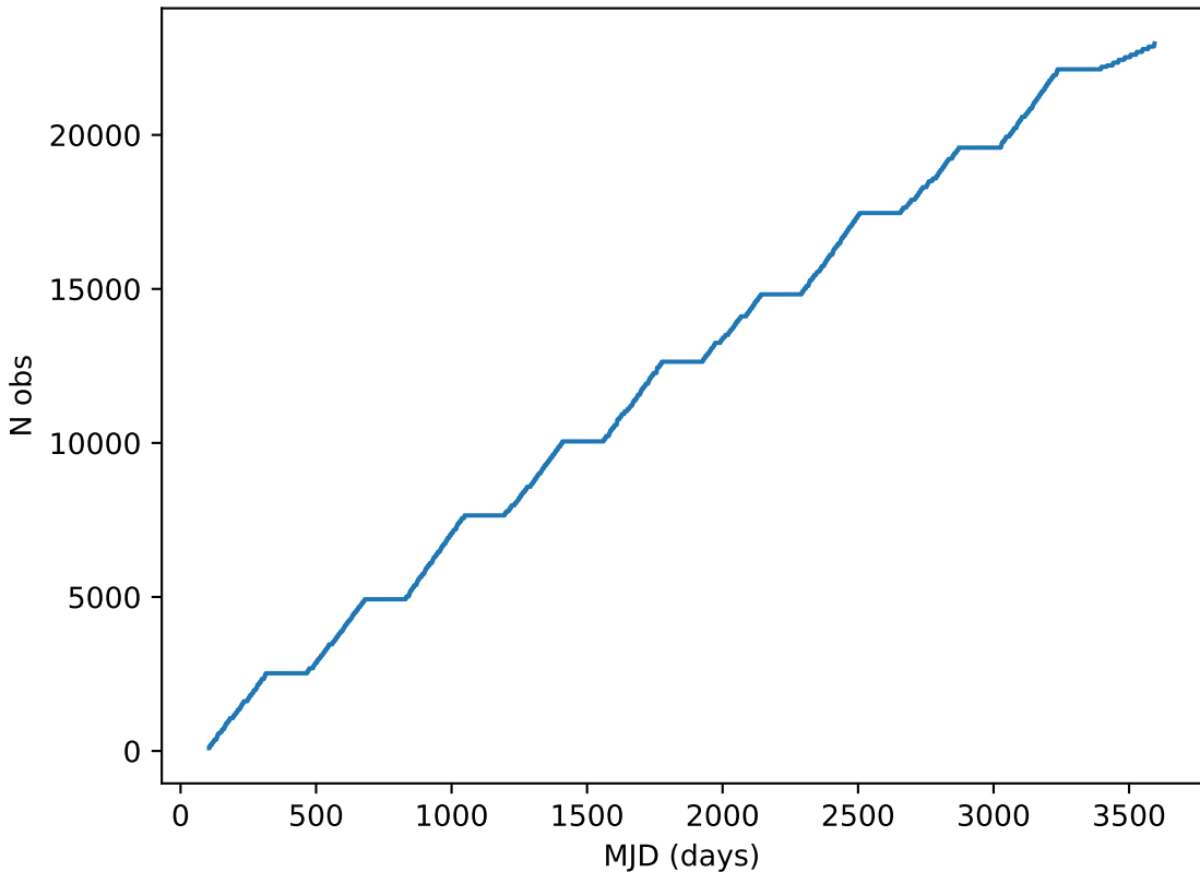
too_elab_r128_d2_griz_v3.4_10yrs all bands: DD:EDFS Cumulative NVisits
