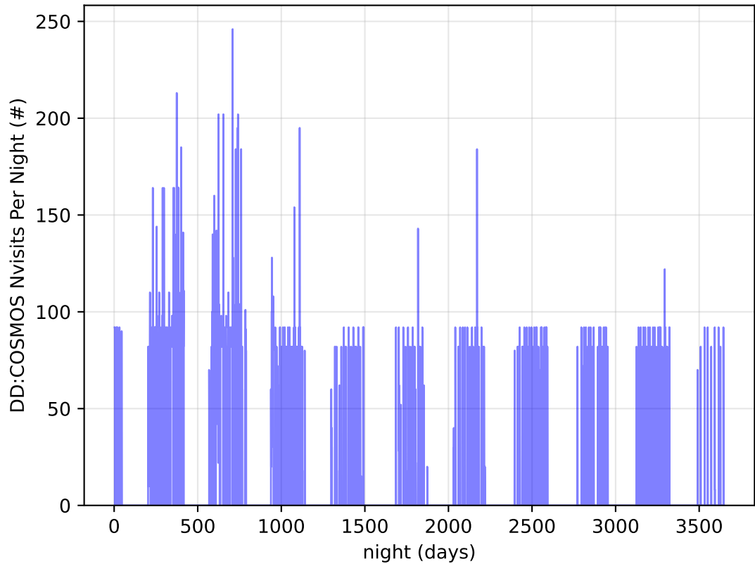
too_elab_r128_d2_griz_v3.4_10yrs all bands: DD: COSMOS Nvisits Per Night
