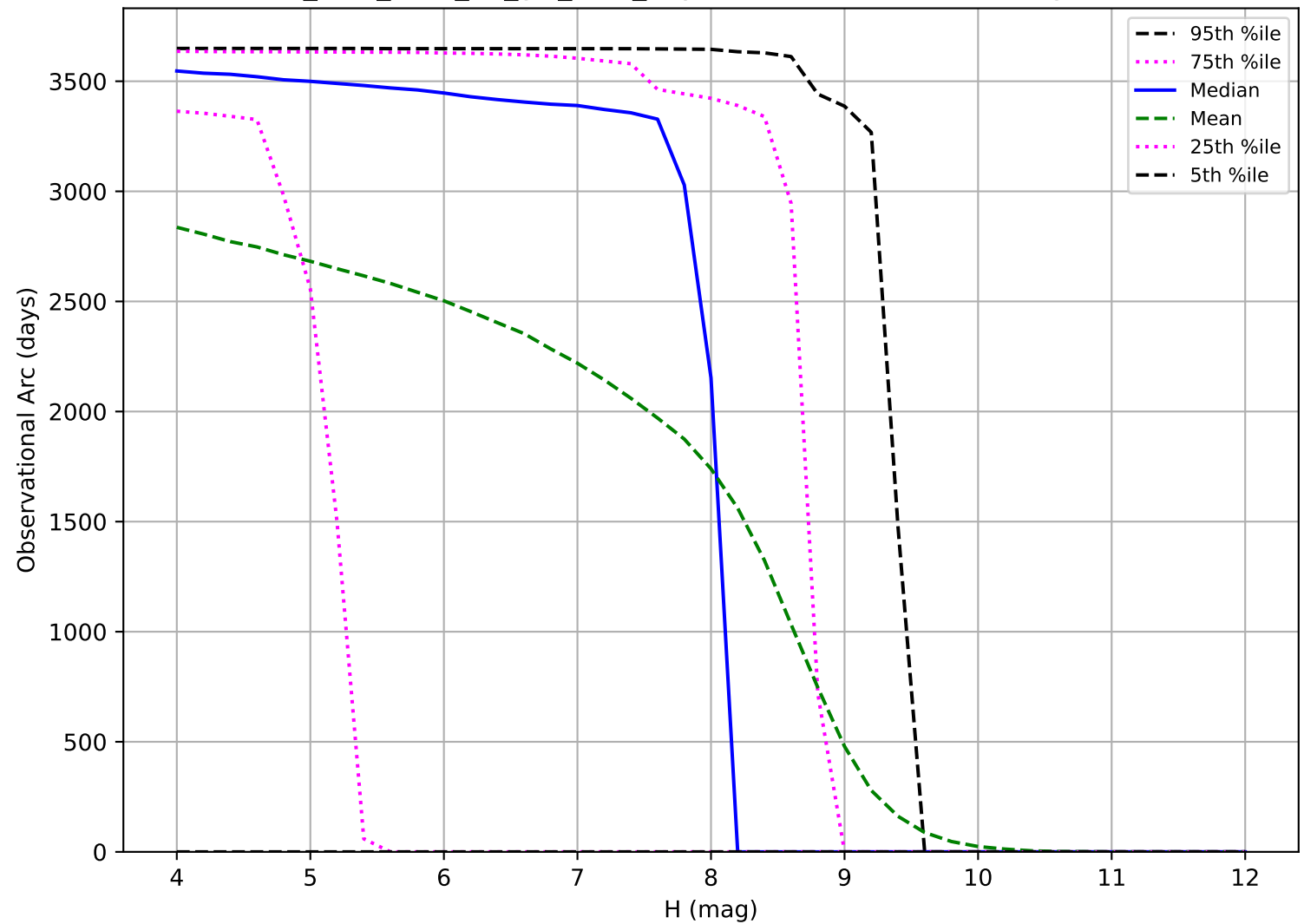
too_elab_r128_d2_giz_v3.4_10yrs: Observational Arc Length TNO
