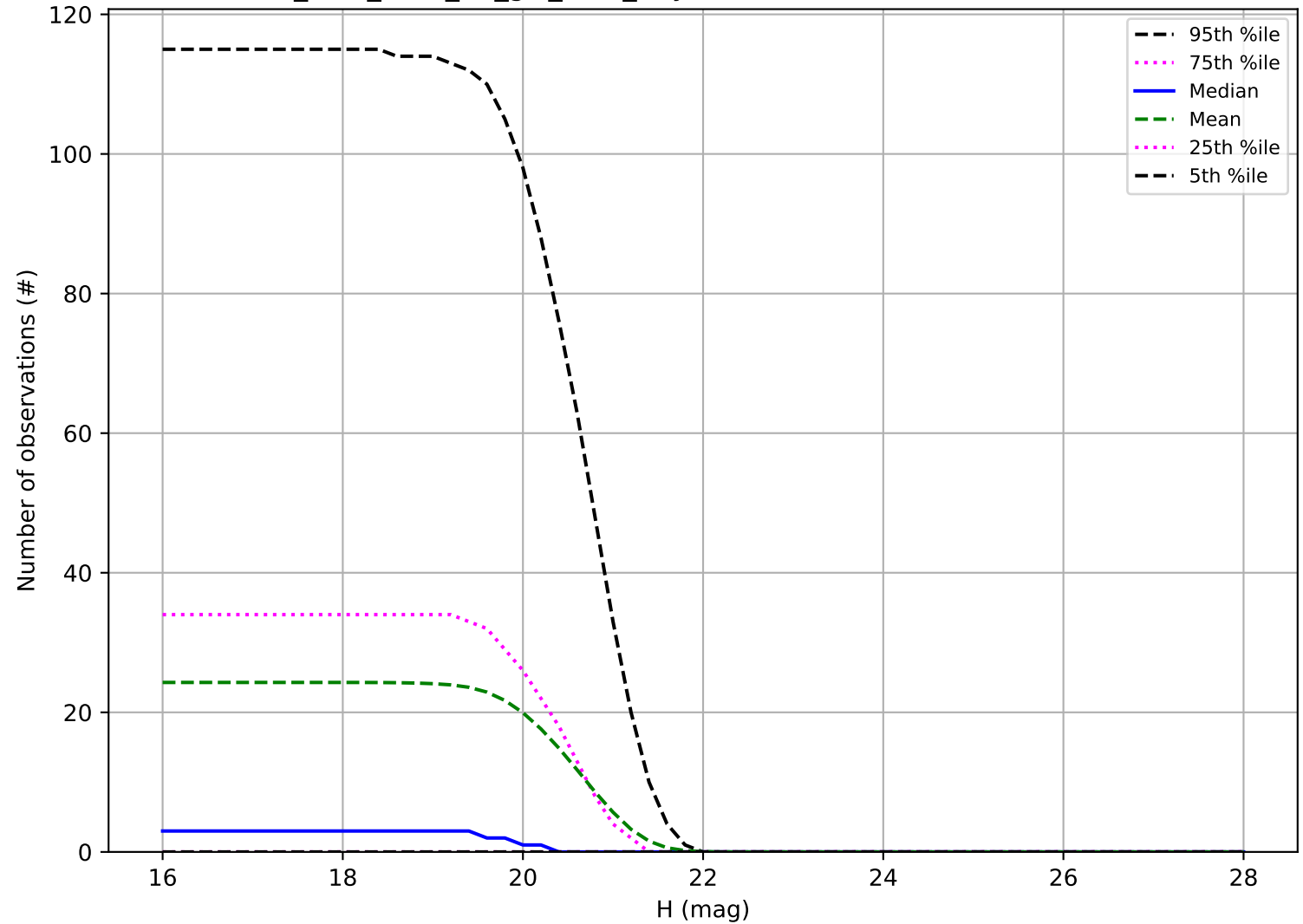
too_elab_r128_d2_giz_v3.4_10yrs: Number of observations Vatira
