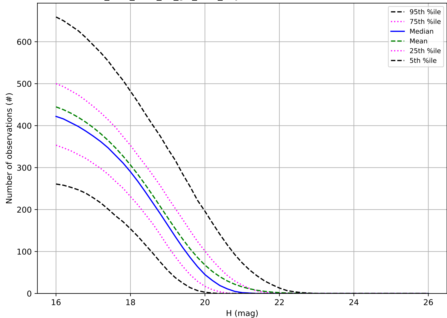
too_elab_r128_d2_giz_v3.4_10yrs: Number of observations MBA
