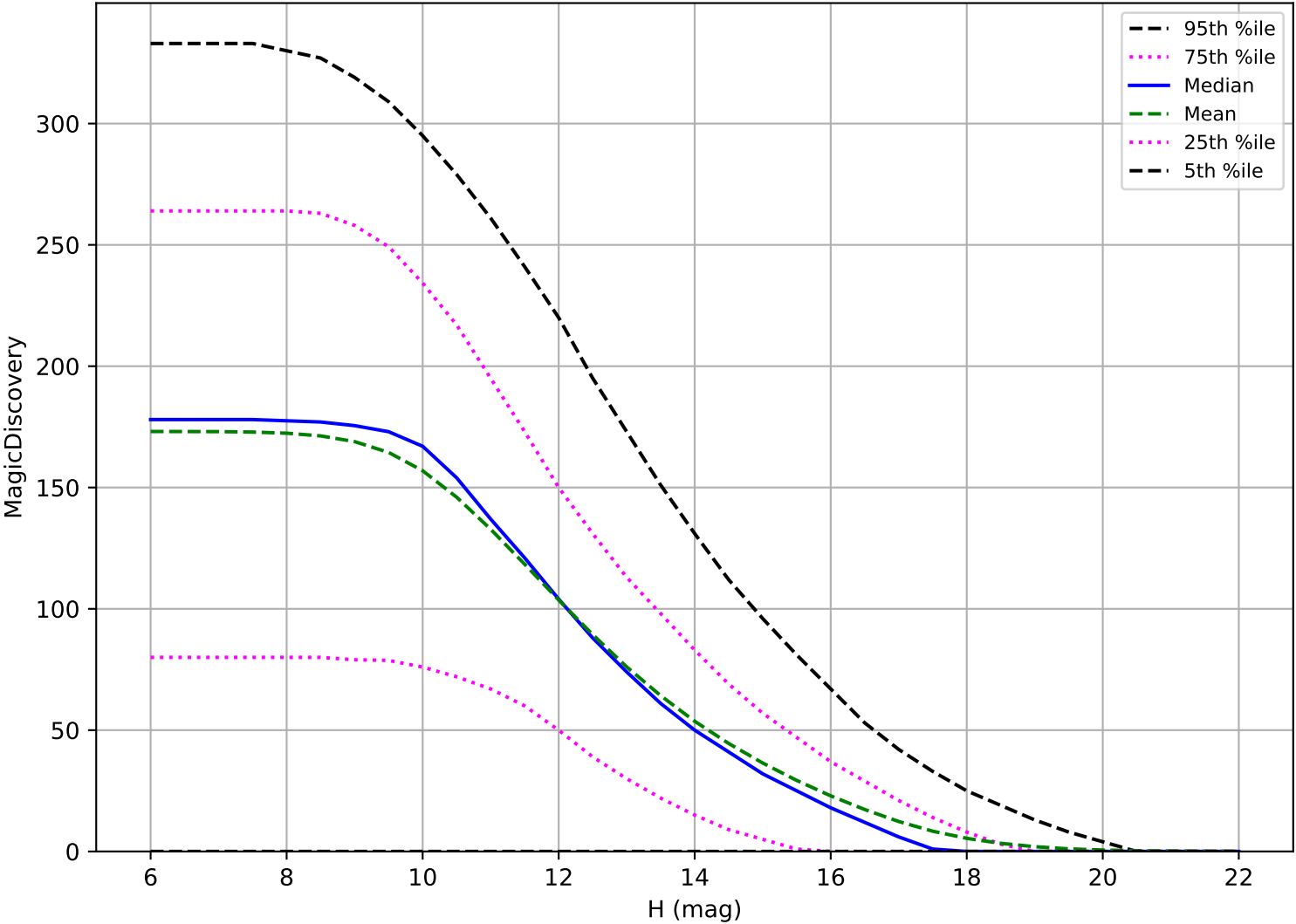
too_elab_r128_d2_giz_v3.4_10yrs: OCC_r5 6 detections in 60 nights detection loss
