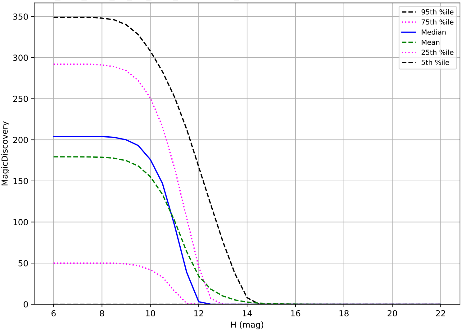
too_elab_r128_d2_giz_v3.4_10yrs: OCC_r20 6 detections in 60 nights detection loss
