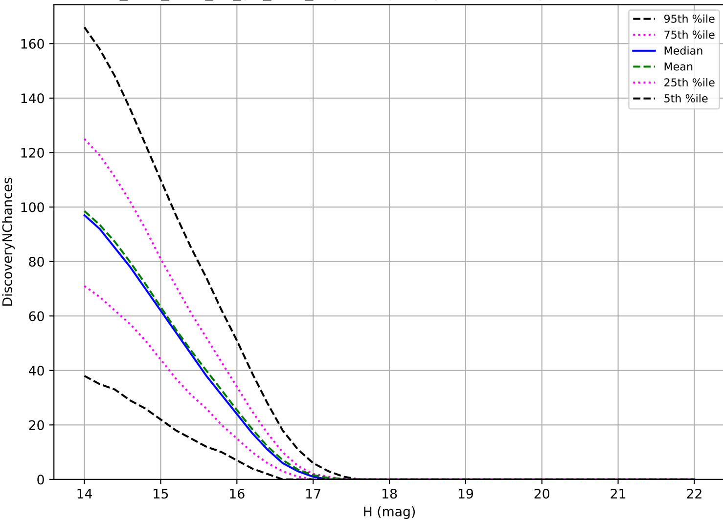
too_elab_r128_d2_giz_v3.4_10yrs: Trojan 3 pairs in 15 nights detection loss
