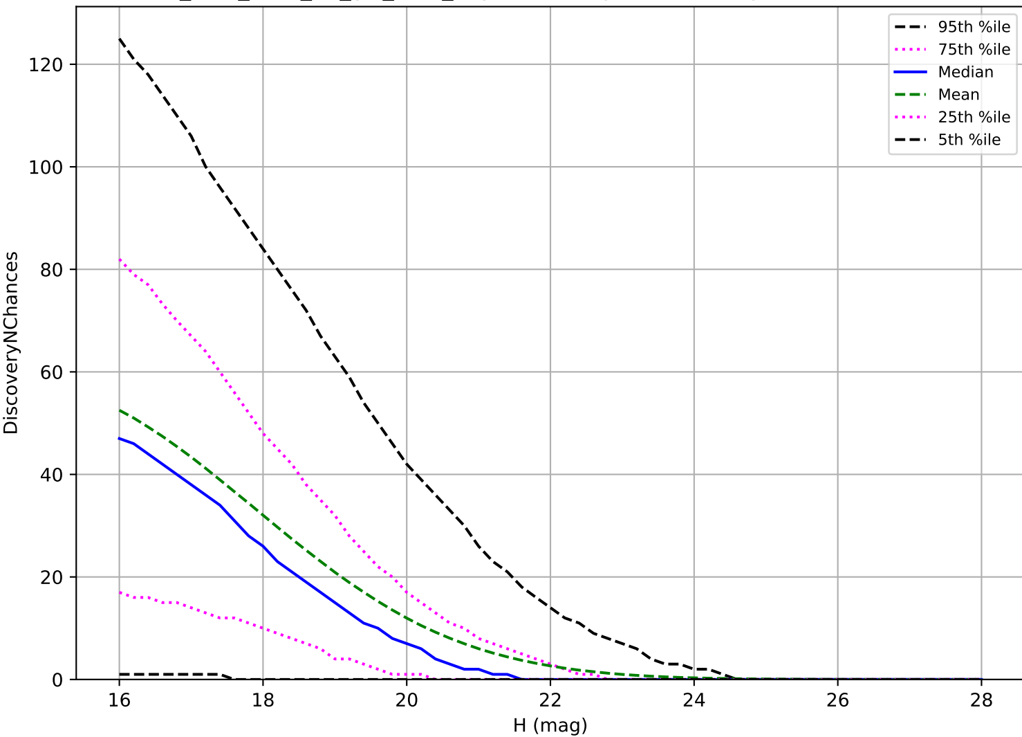
too_elab_r128_d2_giz_v3.4_10yrs: PHA 3 pairs in 15 nights detection loss
