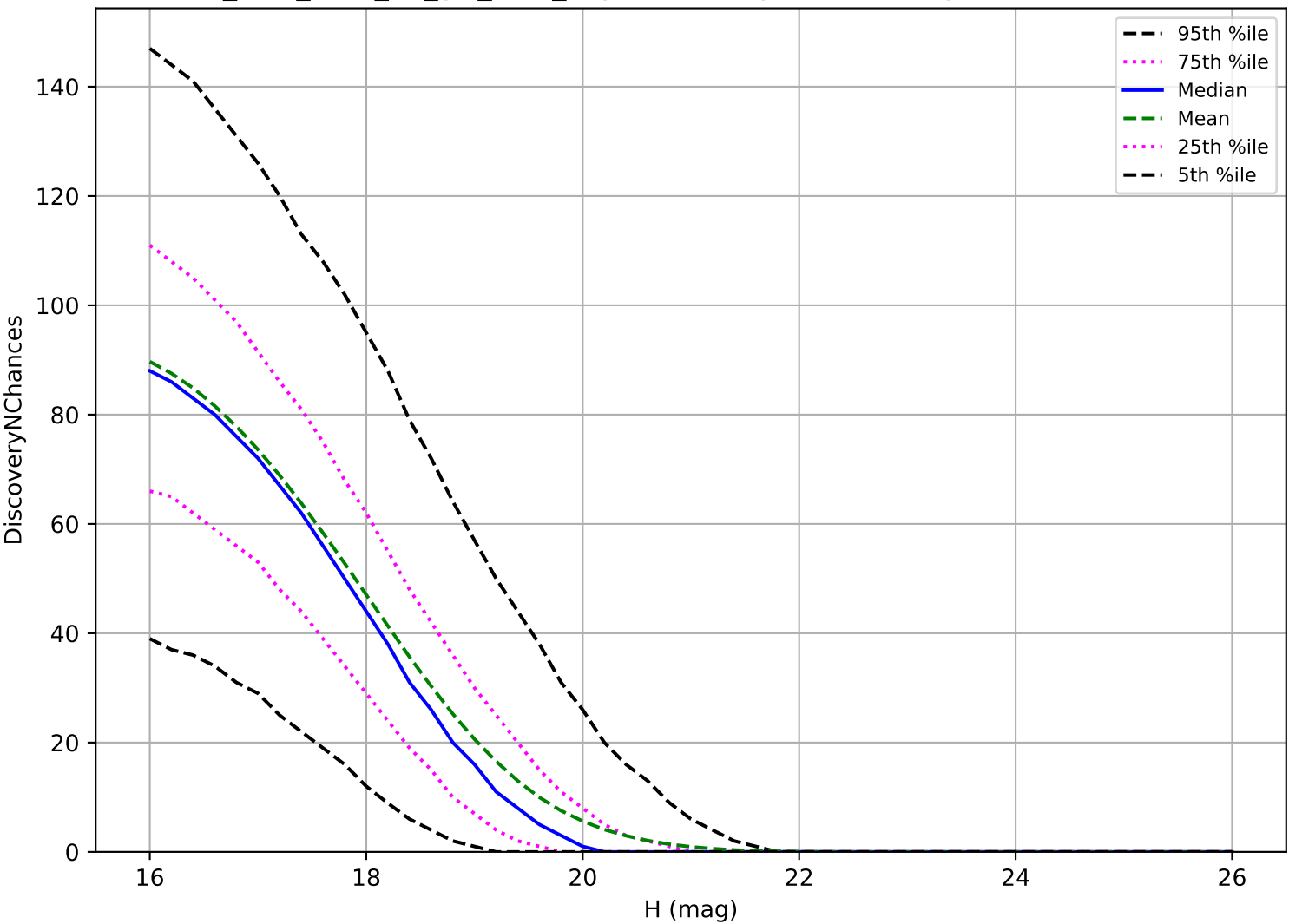
too_elab_r128_d2_giz_v3.4_10yrs: MBA 3 pairs in 15 nights detection loss
