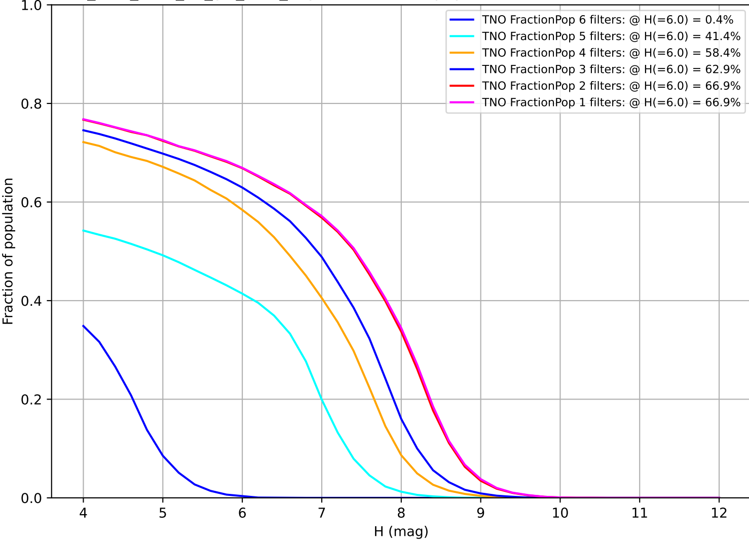
too_elab_r128_d2_giz_v3.4_10yrs: Fraction of population with colors in X filters TNO
