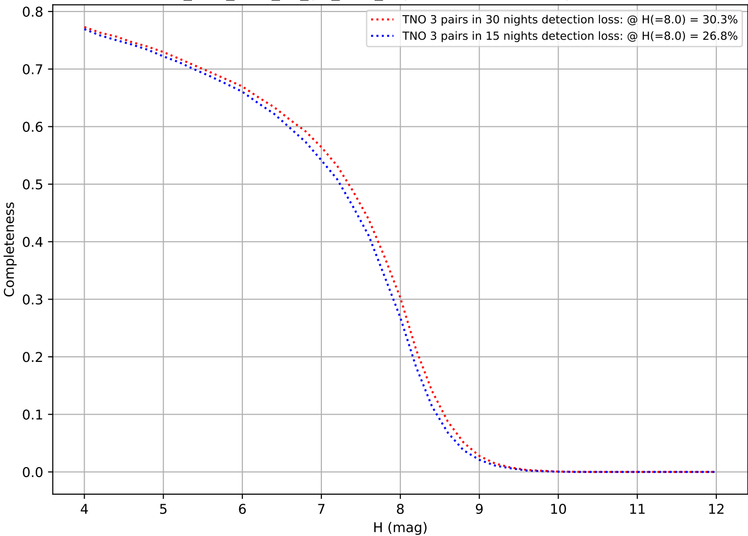
too_elab_r128_d2_giz_v3.4_10yrs: DifferentialCompleteness
