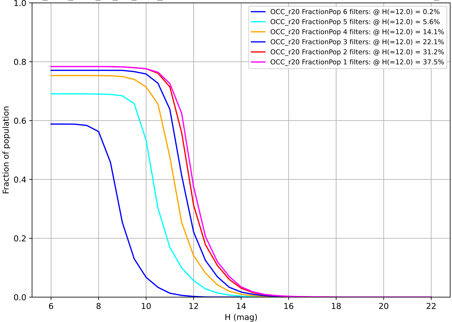
too_elab_r128_d2_giz_v3.4_10yrs: Fraction of population with colors in X filters OCC_r20
