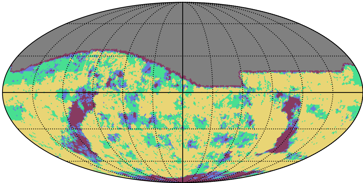
too_elab_r128_d2_giz_v3.4_10yrs g band: YearCoverage night
