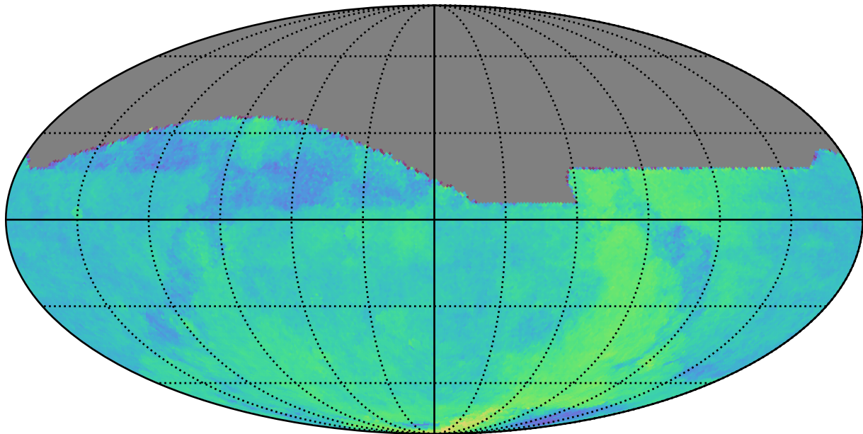
too_elab_r128_d2_giz_v3.4_10yrs : Parallax Coverage @ 24.0
