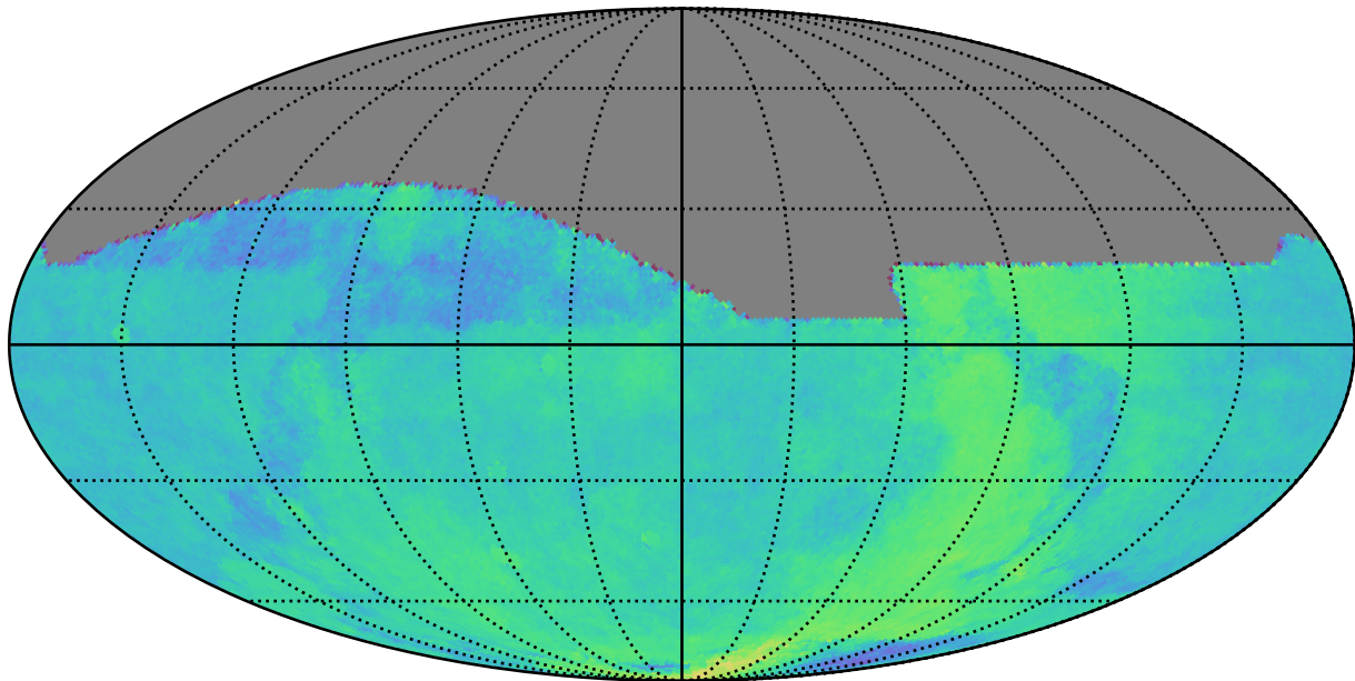
too_elab_r128_d2_giz_v3.4_10yrs : Parallax Coverage @ 22.4
