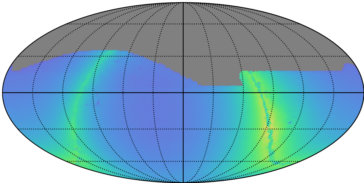
too_elab_r128_d2_giz_v3.4_10yrs i: Nstars_no_crowding
