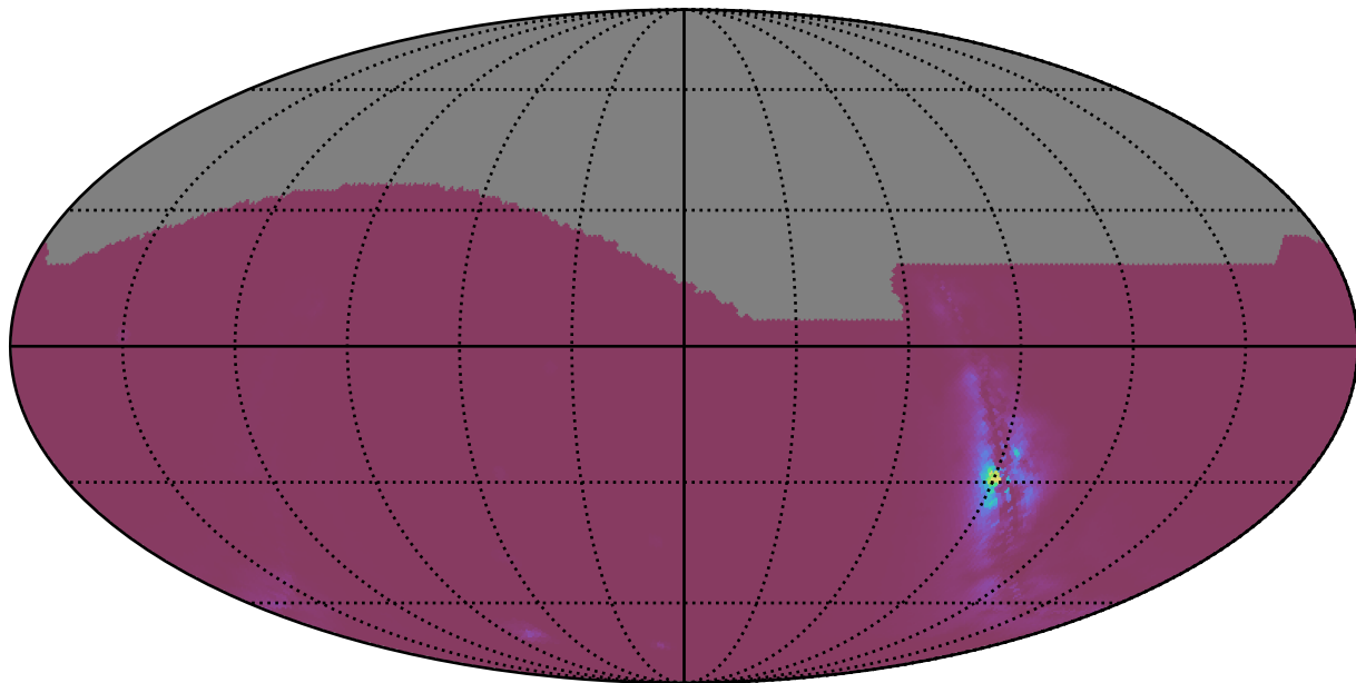
too_elab_r128_d2_giz_v3.4_10yrs : NlcPoints
