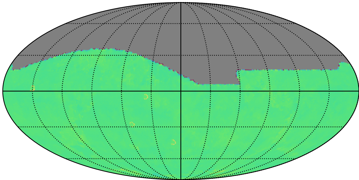
too_elab_r128_d2_giz_v3.4_10yrs r: Kuiper rotTelPos
