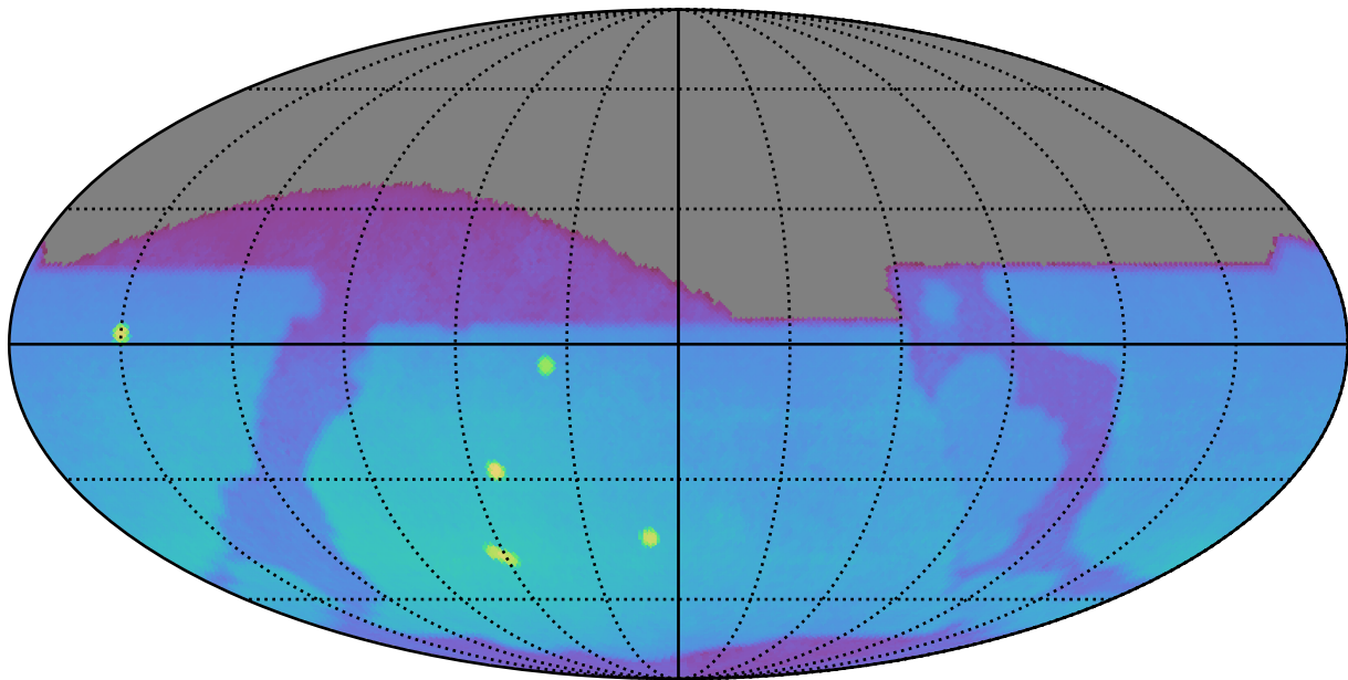
too_elab_r128_d2_giz_v3.4_10yrs : Brown Dwarf, L7
