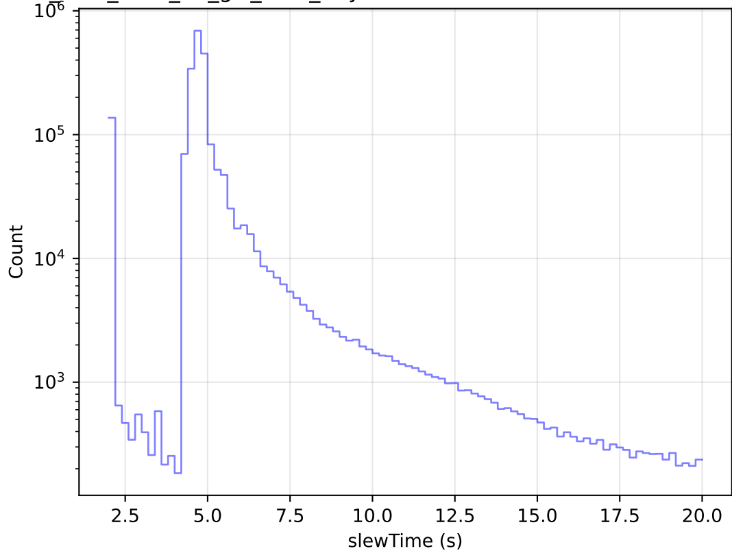
too_elab_r128_d2_giz_v3.4_10yrs All visits: Zoom Slew Time Histogram
