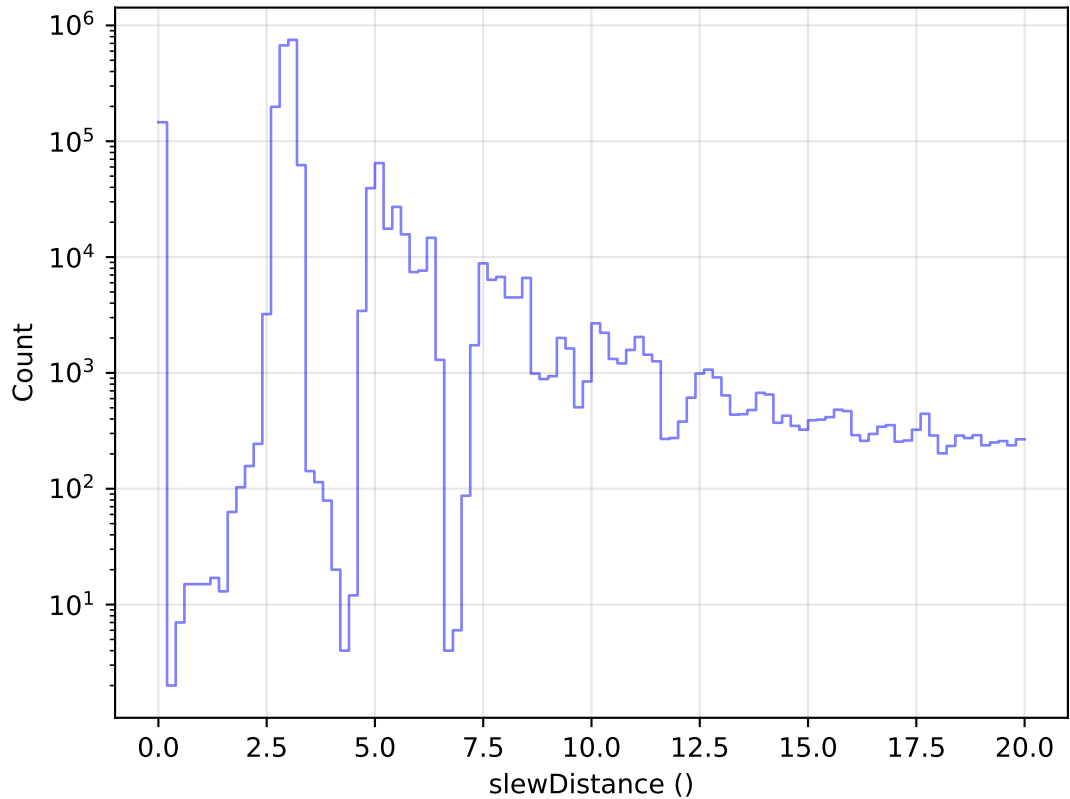
too_elab_r128_d2_giz_v3.4_10yrs All visits: Zoom Slew Distance Histogram
