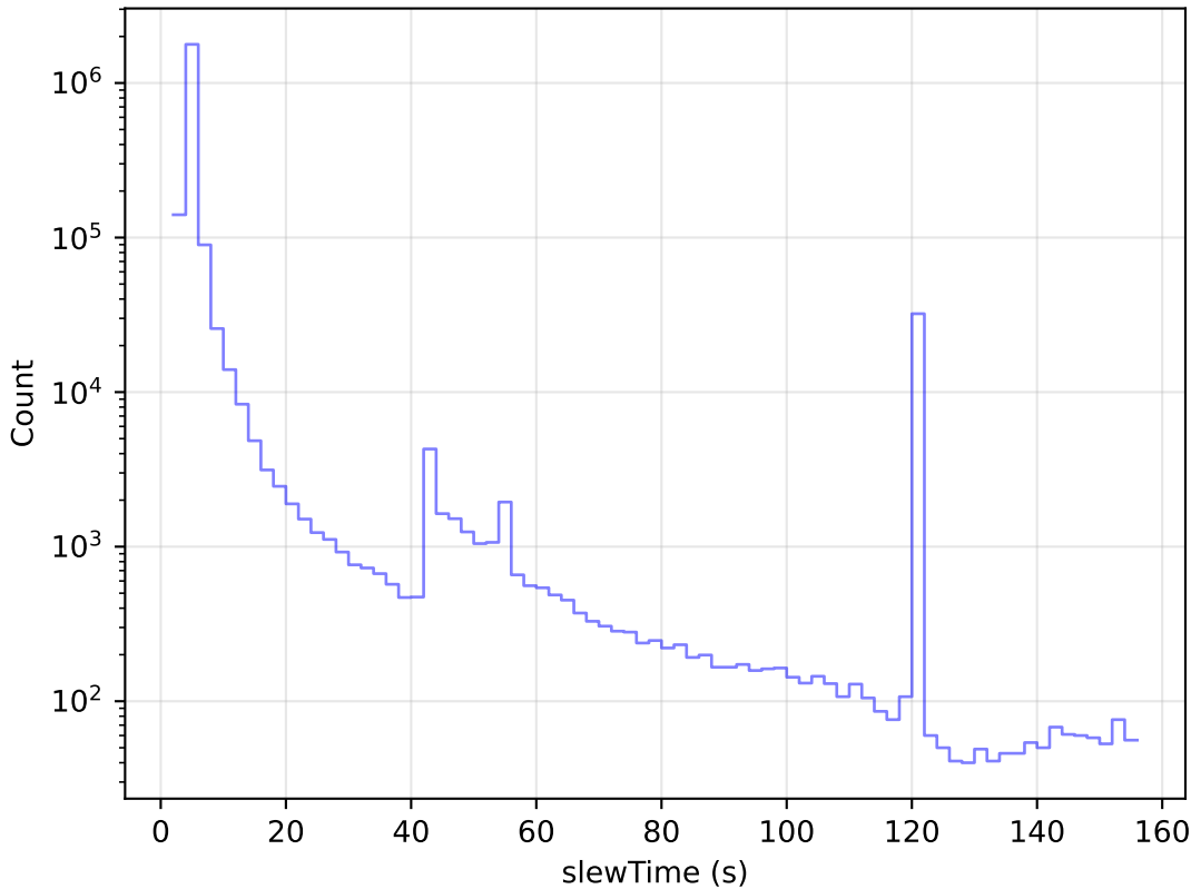
too_elab_r128_d2_giz_v3.4_10yrs All visits: Slew Time Histogram
