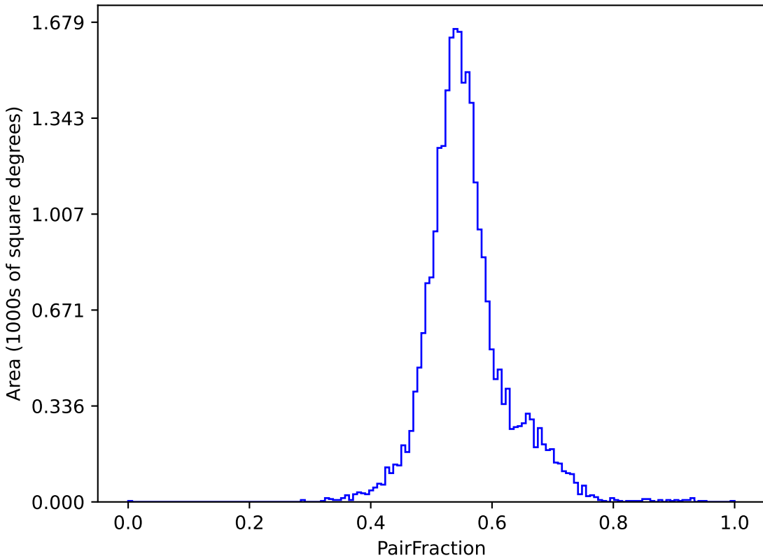
too_elab_r128_d2_giz_v3.4_10yrs (g or r or i): PairFraction
