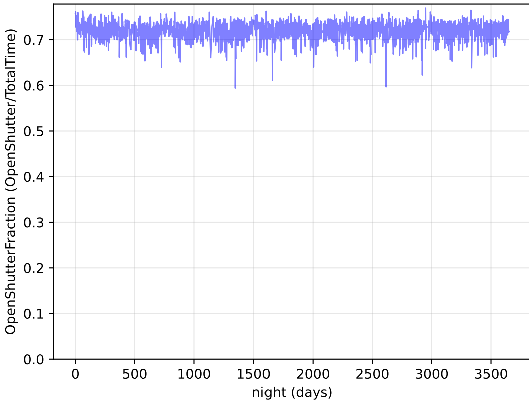
too_elab_r128_d2_giz_v3.4_10yrs : OpenShutterFraction
