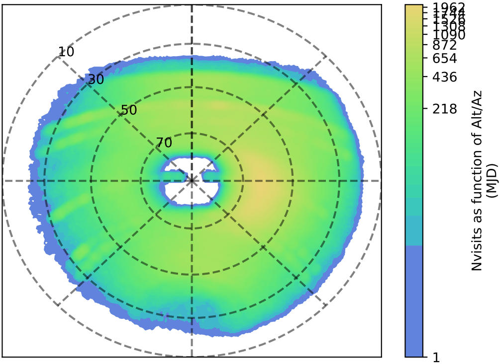
too_elab_r128_d2_giz_v3.4_10yrs y: Nvisits as function of Alt/Az
