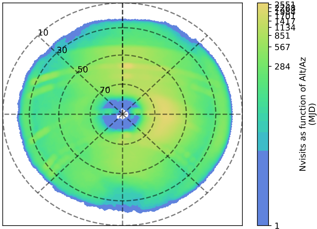
too_elab_r128_d2_giz_v3.4_10yrs i: Nvisits as function of Alt/Az
