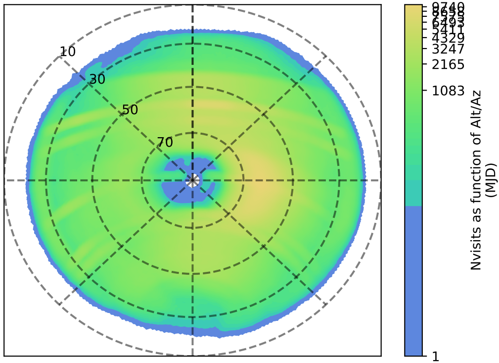
too_elab_r128_d2_giz_v3.4_10yrs : Nvisits as function of Alt/Az
