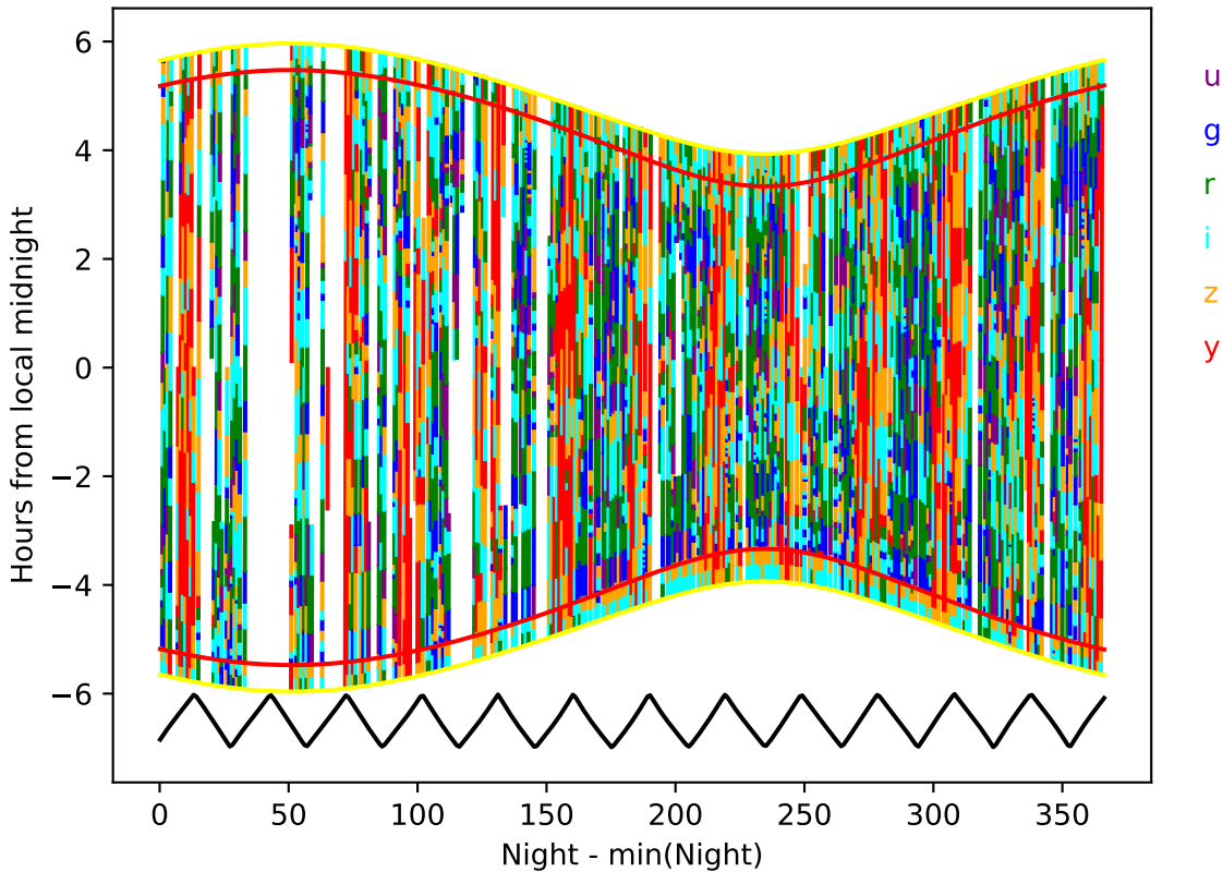
too_elab_r128_d2_giz_v3.4_10yrs year 8-9: Hourglass
