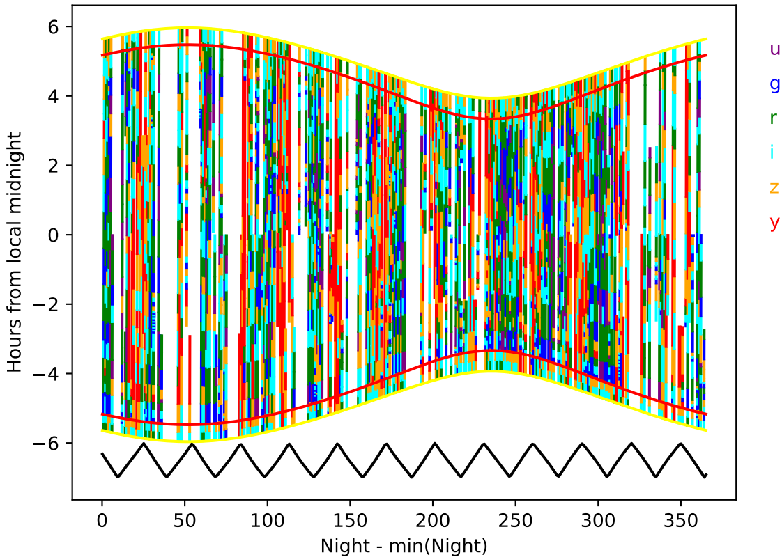
too_elab_r128_d2_giz_v3.4_10yrs year 7-8: Hourglass
