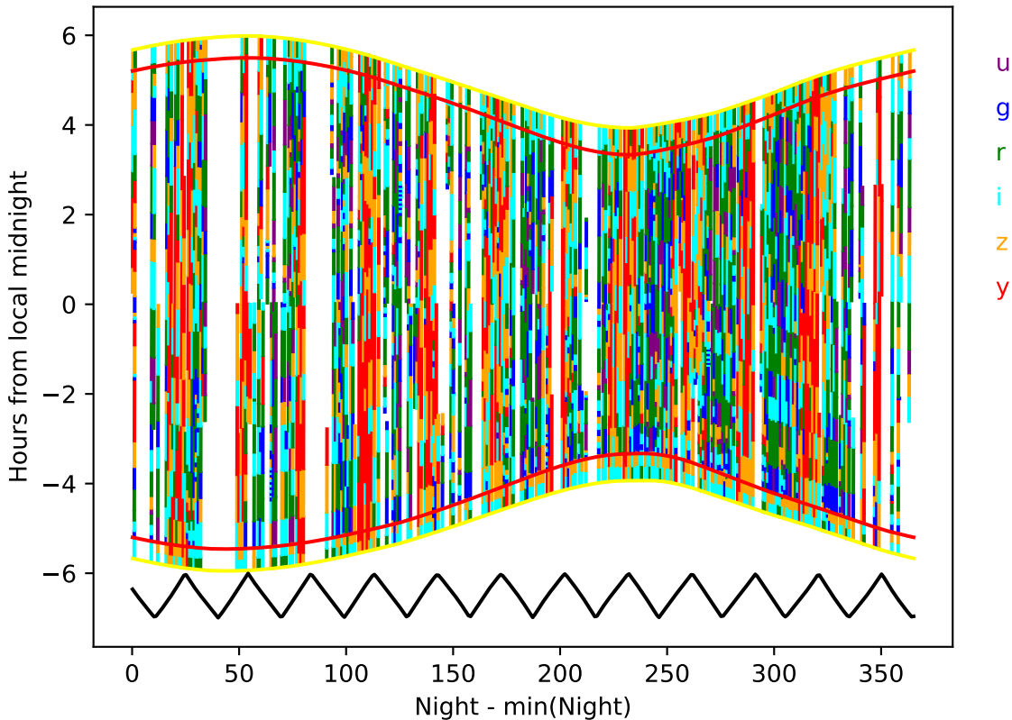
too_elab_r128_d2_giz_v3.4_10yrs year 4-5: Hourglass
