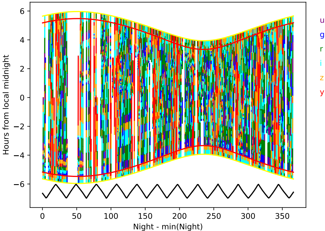
too_elab_r128_d2_giz_v3.4_10yrs year 2-3: Hourglass
