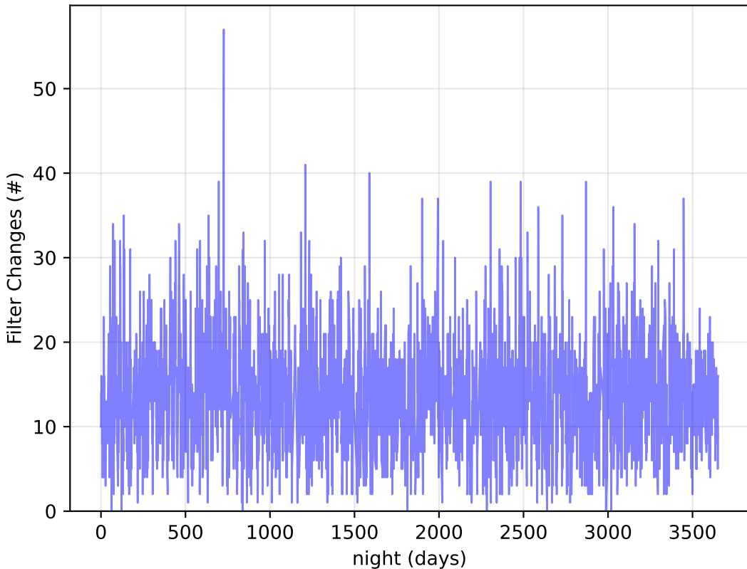
too_elab_r128_d2_giz_v3.4_10yrs : Filter Changes
