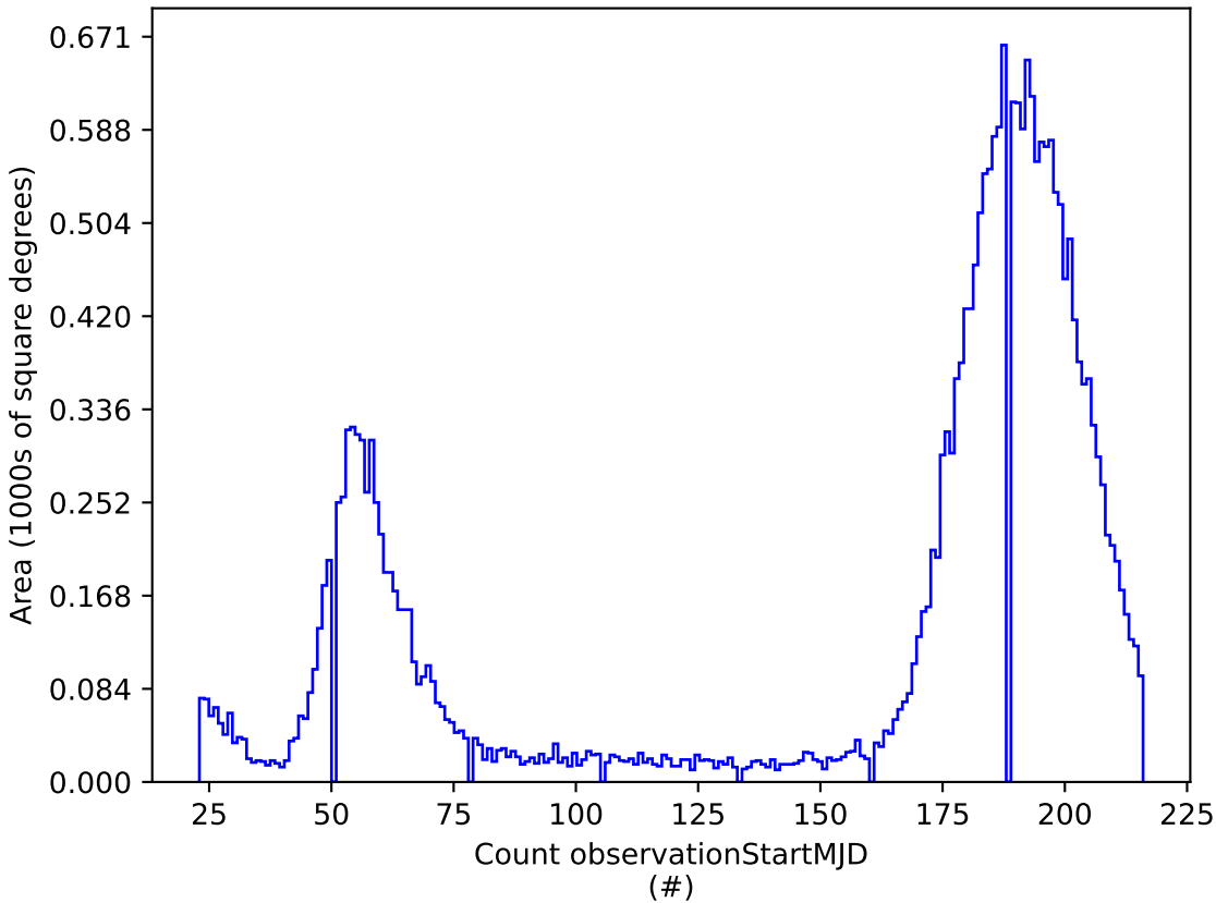
too_elab_r128_d2_giz_v3.4_10yrs i: Count observationStartMJD
