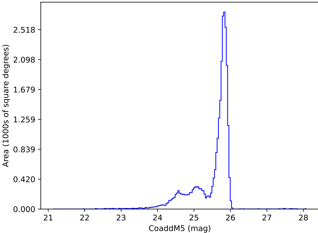
too_elab_r128_d2_giz_v3.4_10yrs z: CoaddM5
