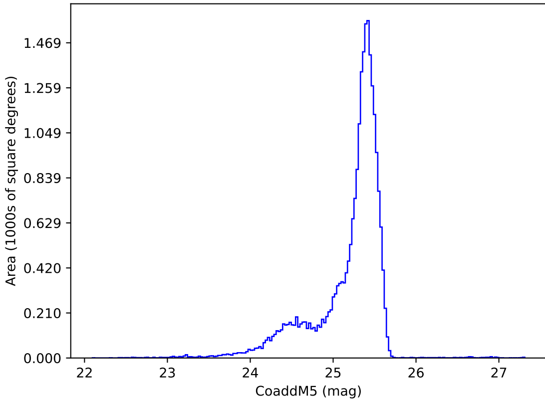
too_elab_r128_d2_giz_v3.4_10yrs u: CoaddM5
