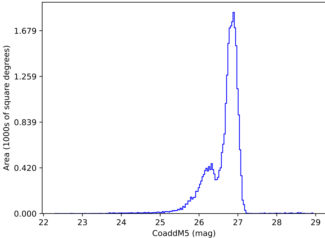
too_elab_r128_d2_giz_v3.4_10yrs g: CoaddM5
