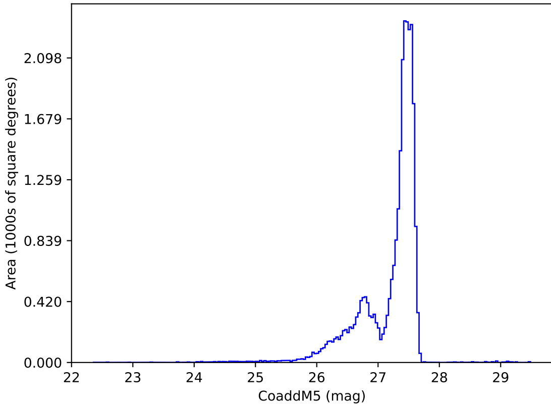
too_elab_r128_d2_giz_v3.4_10yrs : CoaddM5
