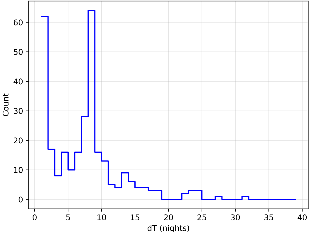
too_elab_r128_d2_giz_v3.4_10yrs all bands: DD:XMM_LSS Delta Nights Histogram
