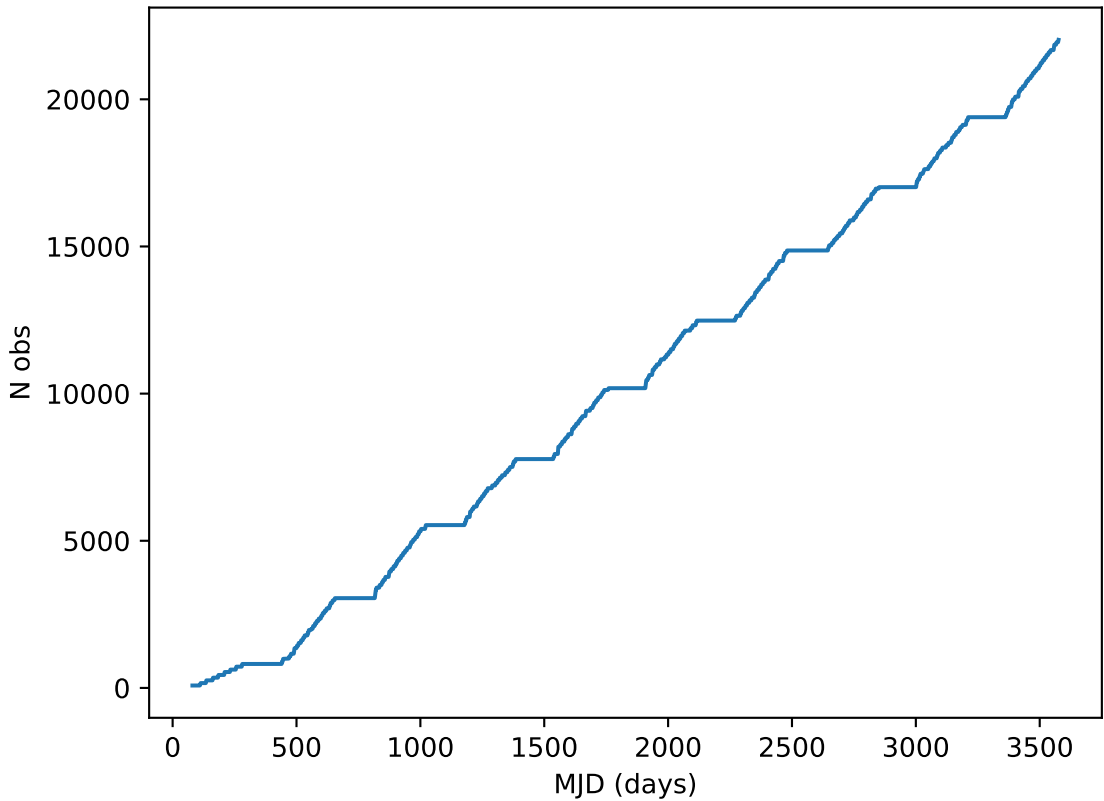
too_elab_r128_d2_giz_v3.4_10yrs all bands: DD:XMM_LSS Cumulative NVisits
